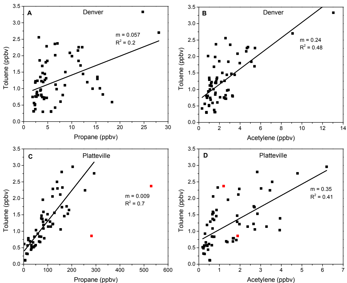
Figure S1. Correlations of toluene with propane and acetylene.
