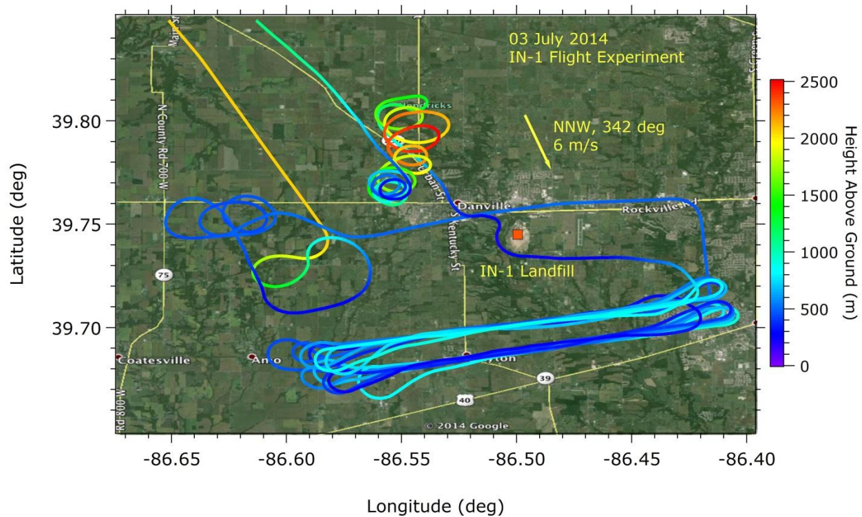
Figure S2. Experimental flight path as a function of altitude on 03 July 2014 at the IN-1 Landfill site. Horizontal transects were flown at 4.5 km and 6 km downwind distances. Winds were from the North Northwest ( 342^\circ \pm 18^\circ ) at 6.2 \pm 2.0 ( 1\sigma ) \text{ms}^{-1} .
