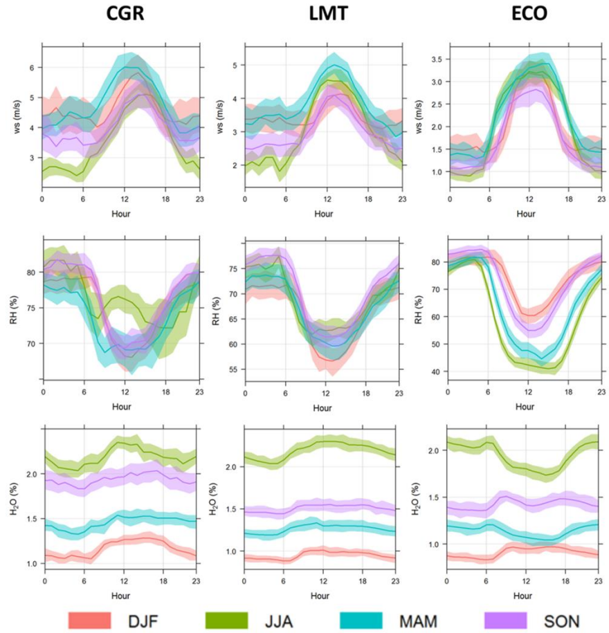
Figure S1. Seasonal average diurnal variation of wind speed (WS), relative humidity (RH) and water vapor ( H_2O ) at the three I-AMICA sites. Dashed areas denote the 96% confidence levels. Time is expressed in local time (UTC+1).
