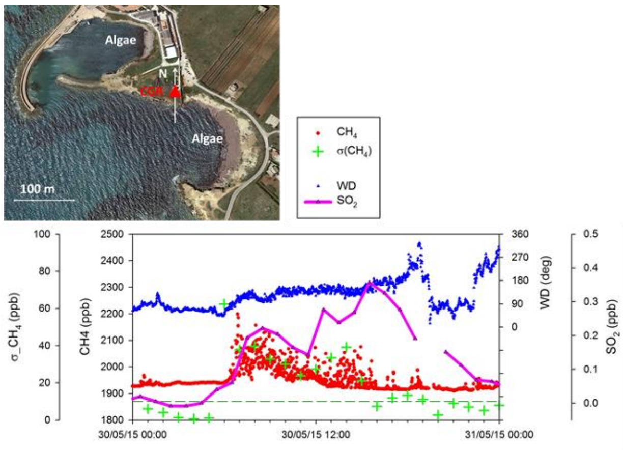
Figure S3. Satellite image (courtesy of Google Earth) of the CGR location. The two small bays with alga accumulation are reported together with CGR location (red triangle). Below a representative event with concurrent CH 4 and SO 2 enhancements under south-easterly wind (i.e. from the bay) is shown.
