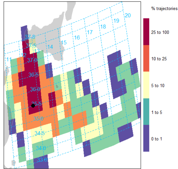
Figure S4. Patterns of air-masses moving from CGR to LMP during the investigated period. Frequency spatial distribution of HYSPLIT back-trajectory points for the air-mass transport events from CGR (black star) to LMP (black dot).
