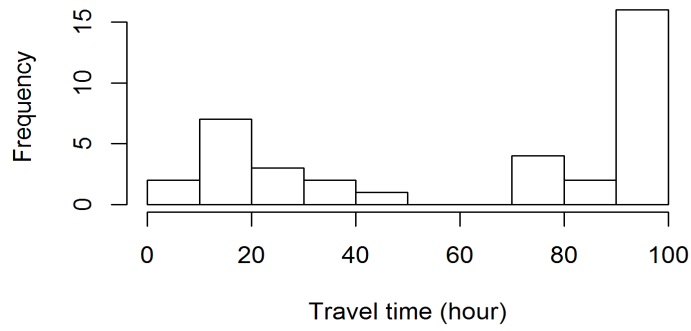
Figure S5. Histogram of the frequency distribution of travel times for air-masses from CGR to LMP.
