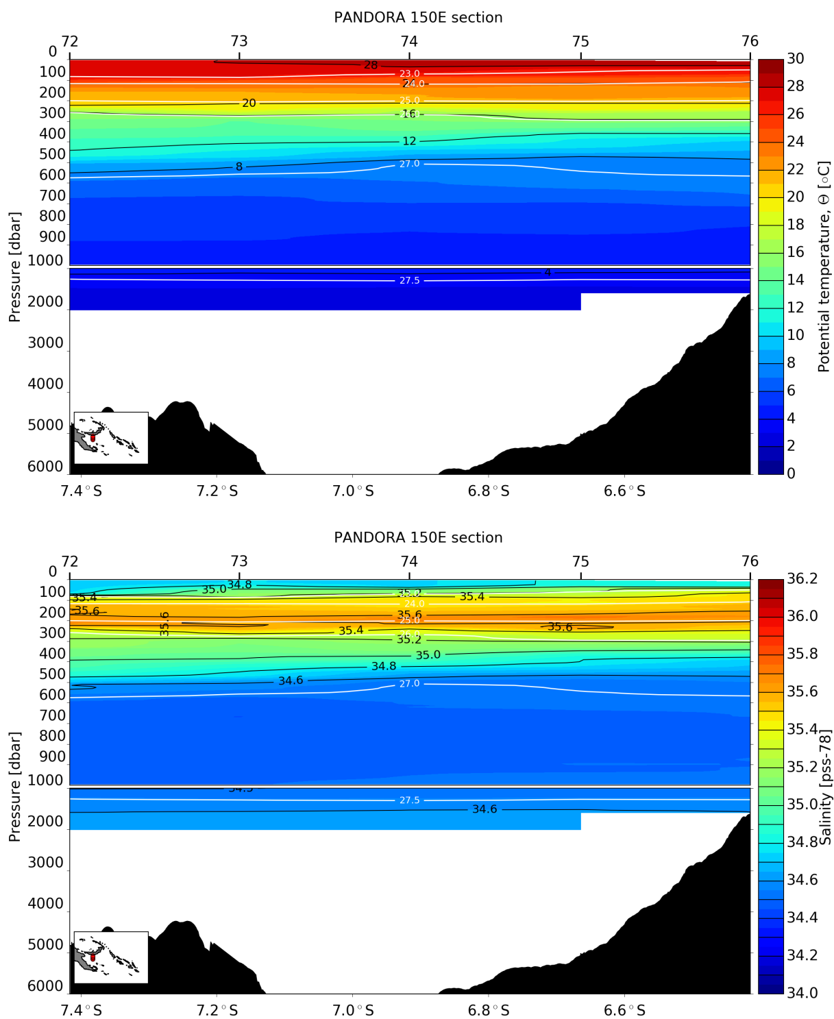
Figure S13: (Upper) potential temperature and (lower) salinity section along 150E
