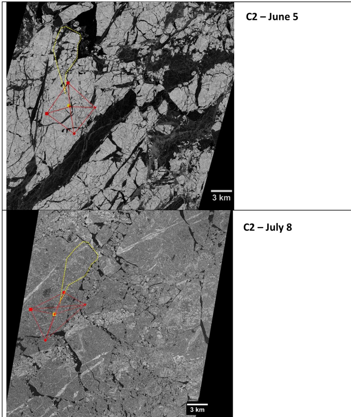
Figure S1. A sequence of TS-X SM images showing the transition of an ice floe. The ice floe is marked with yellow dashed polygon, which has been broken apart during mid-August breakup (see Figure 15).
