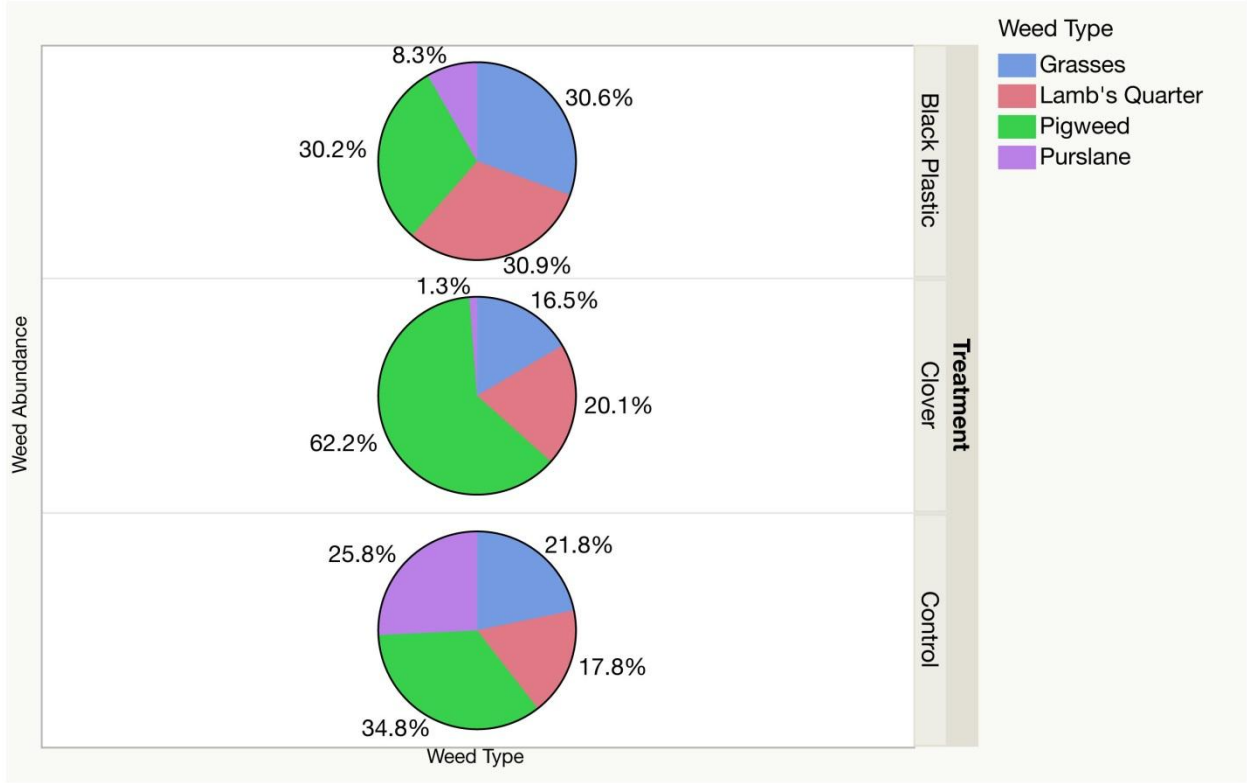
Figure S3. Abundance of Weed Type in a Tomato Cropping System on the Basis of Weed Suppression Treatment. The abundance of weed type (grasses, lamb’s quarter, pigweed, and purslane) varied across the three weed suppression strategies in the tomato cropping system.
