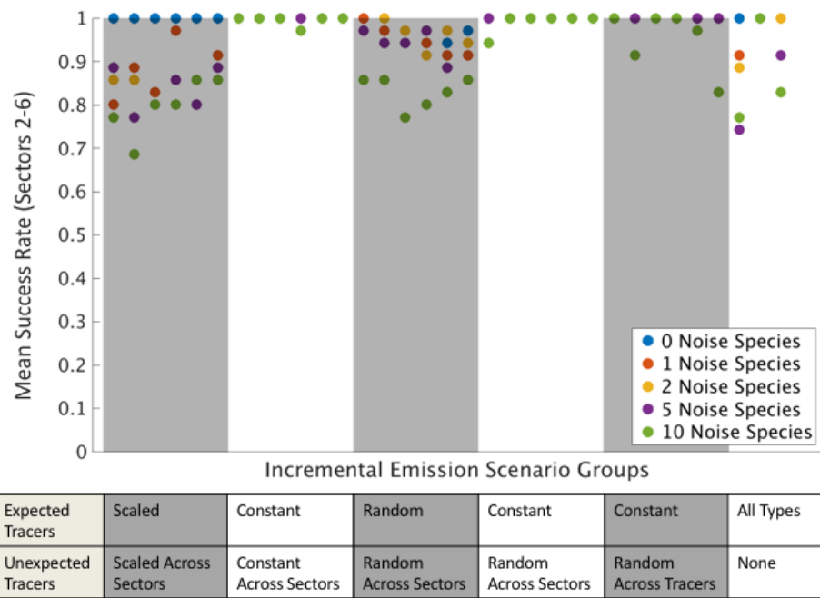
Figure S11. A noise-scenario comparison of the control case as in Figure 7, but for the Success Rate metric.
