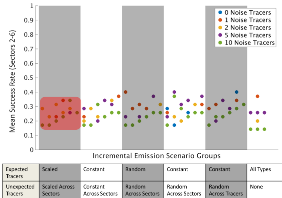
Figure S13. A noise-scenario comparison of the case with the domain-filling problem as in Figure 8, but for the Success Rate metric.
