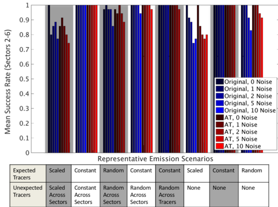
Figure S15. The “all towers” comparison in the control scenario as in Figure 9, but using the Success Rate metric.
