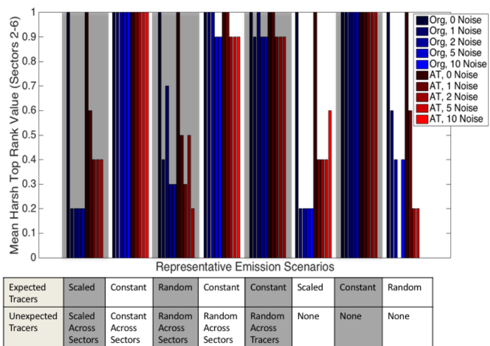
Figure S16. The “all towers” comparison in the control scenario as in Figure 9, but using the Harsh Top Rank metric.
