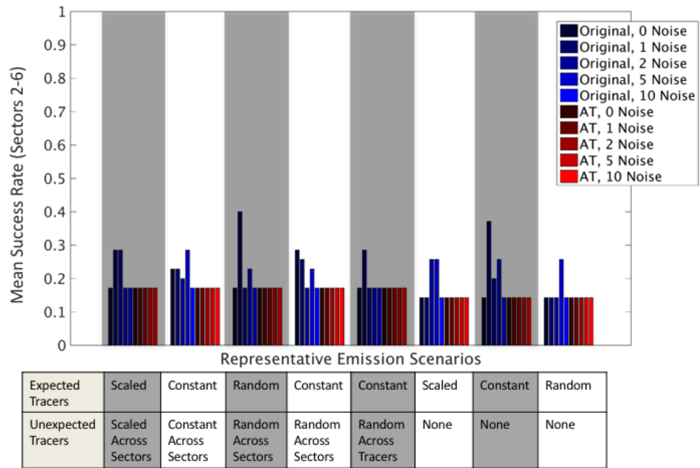
Figure S17. The “all towers” comparison in the scenario with the domain-filling problem, as in Figure 10, but using the Success Rate metric.
