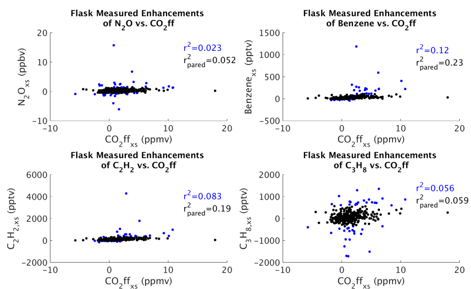
Figure S2. Scatter plots for the raw data from several measured flask species against CO_2ff with the corresponding r^2 value. r_{pared}^2 was computed by removing the top and bottom 5% of values from the non- CO_2ff species.
