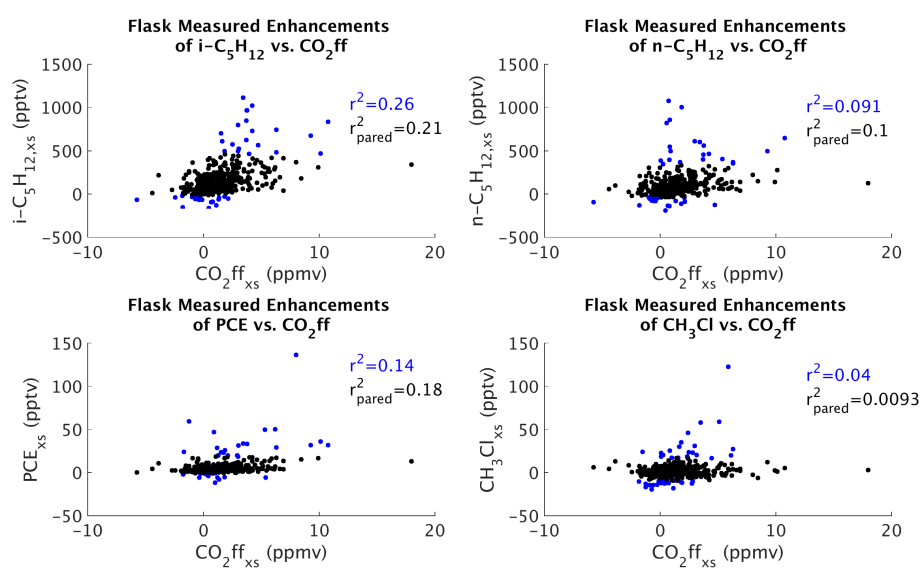
Figure S3. Scatter plots for the raw data from several measured flask species against CO_2ff with the corresponding r^2 value. r^2_{pared} was computed by removing the top and bottom 5% of values from the non- CO_2ff species.
