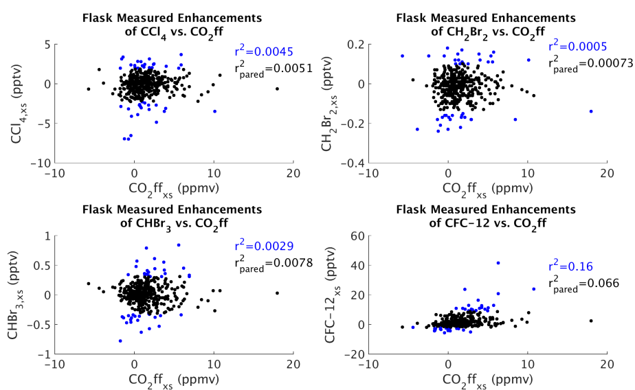
Figure S5. Scatter plots for the raw data from several measured flask species against CO_2ff with the corresponding r^2 value. r^2_{pared} was computed by removing the top and bottom 5% of values from the non- CO_2ff species.
