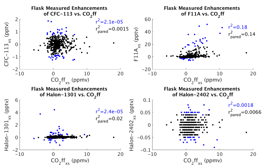
Figure S6. Scatter plots for the raw data from several measured flask species against CO_2ff with the corresponding r^2 value. r_{pared}^2 was computed by removing the top and bottom 5% of values from the non- CO_2ff species.
