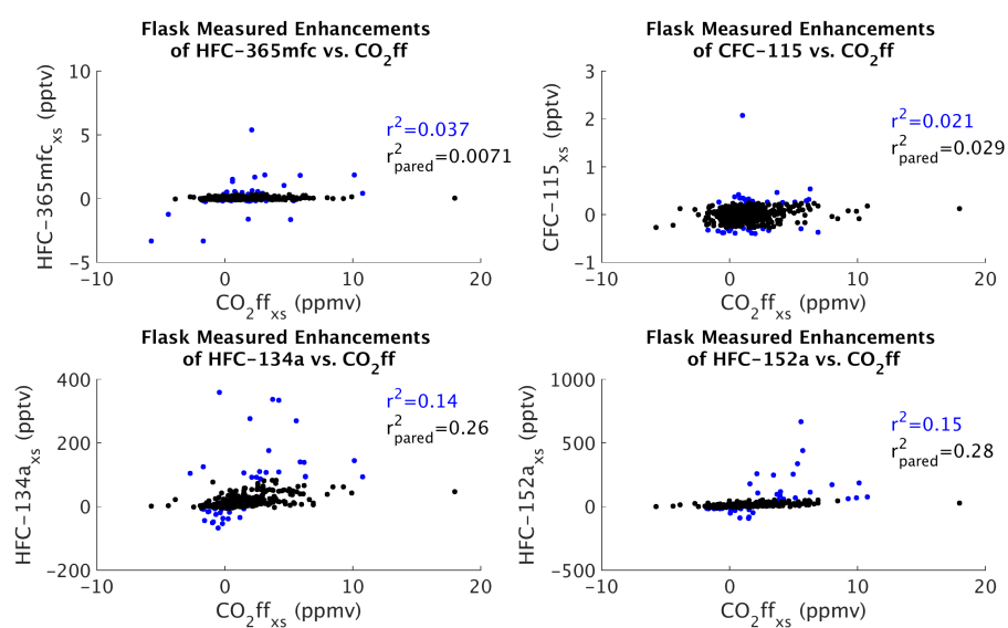
Figure S7. Scatter plots for the raw data from several measured flask species against CO_2ff with the corresponding r^2 value. r^2_{pared} was computed by removing the top and bottom 5% of values from the non- CO_2ff species.
