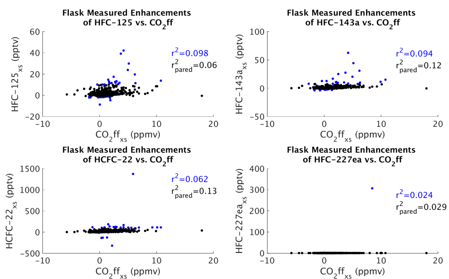
Figure S8. Scatter plots for the raw data from several measured flask species against CO_2ff with the corresponding r^2 value. r_{pared}^2 was computed by removing the top and bottom 5% of values from the non- CO_2ff species.
