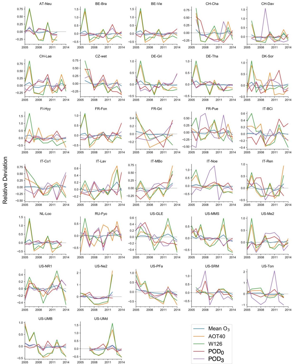
Figure S1. Time series (2005-2014) of ozone flux and concentration at all sites. Values are shown as relative deviation from the ten-year mean of each metric at each site ( \text{value}/\text{mean} - 1 ).
